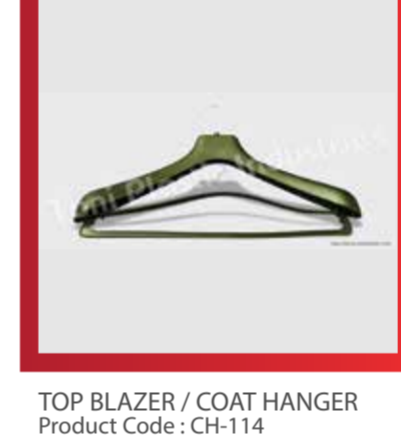
TOP BLAZER / COAT HANGER Product Code : CH-114 LENGTH - 455 MM HEIGHT - 270 MM WIDTH - 10 MM INNER GAP - 120 MM
