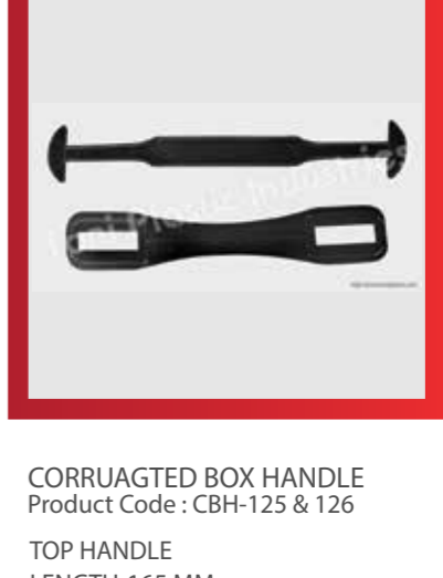
CORRUGATED BOX HANDLE Product Code: CBH-125 & 126 TOP HANDLE - 165 MM LENGTH - 165 MM WIDTH - 15 MM BOTTOM HANDLE - 140 MM LENGTH - 140 MM HOLE GAP - 85 MM
