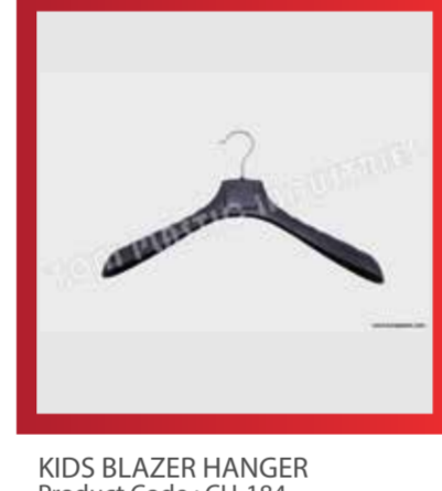
KIDS BLAZER HANGER Product Code : CH-184 LENGTH - 350 MM HEIGHT - 120 MM WIDTH - 50 MM INNER GAP - 75 MM
