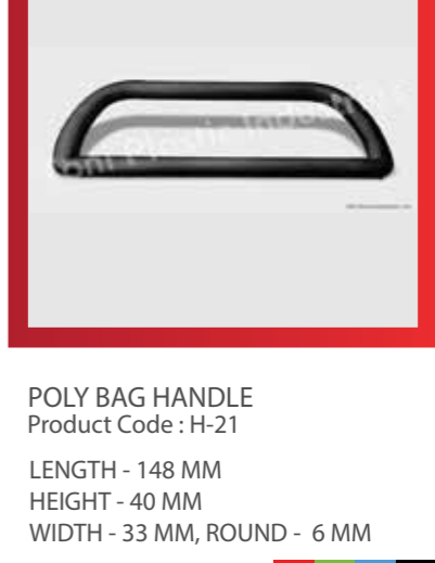
POLY BAG HANDLE Product Code: H-21 LENGTH - 140 MM HEIGHT - 40 MM WIDTH - 33 MM, ROUND - 6 MM
