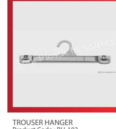
TROUSER HANGER Product Code : BH-103 LENGTH - 300 MM HEIGHT - 90 MM WIDTH - 23 MM
