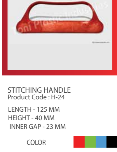
STITCHING HANDLE Product Code: H-24 LENGTH - 125 MM HEIGHT - 40 MM INNER GAP - 23 MM
