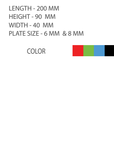
DIAMOND DOWEL SLEEVE Product Code: D-1H LENGTH - 200 MM HEIGHT - 90 MM WIDTH - 40 MM PLATE SIZE - 6 MM & 8 MM
