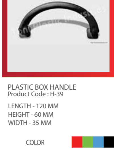
PLASTIC BOX HANDLE Product Code: H-39 LENGTH - 120 MM HEIGHT - 60 MM WIDTH - 35 MM
