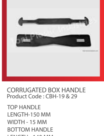
CORRUGATED BOX HANDLE Product Code: CBH-19 & 29 TOP HANDLE - 150 MM LENGTH - 150 MM WIDTH - 15 MM BOTTOM HANDLE - 140 MM LENGTH - 140 MM HOLE GAP - 85 MM
