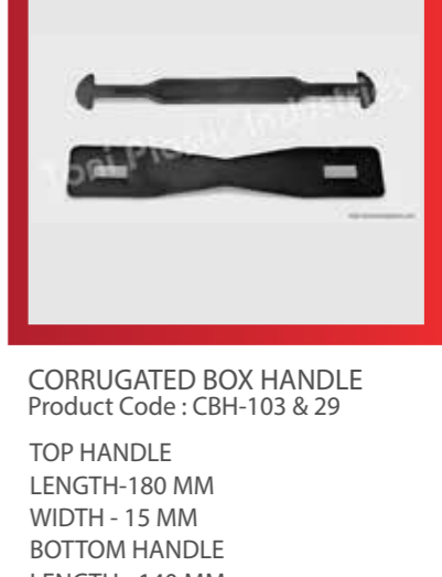
CORRUGATED BOX HANDLE Product Code: CBH-103 & 29 TOP HANDLE - 180 MM LENGTH - 180 MM WIDTH - 15 MM BOTTOM HANDLE - 140 MM LENGTH - 140 MM HOLE GAP - 85 MM
